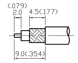
STRIPPING DIMENSION
