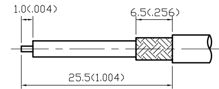
STRIPPING DIMENSION
