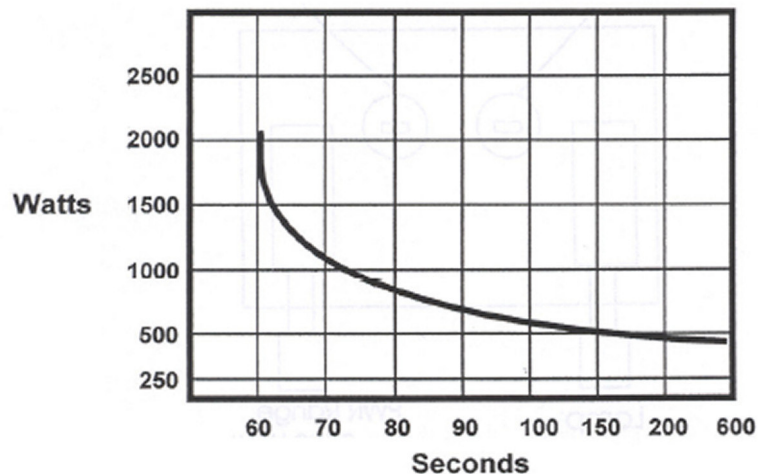
Power Capability
